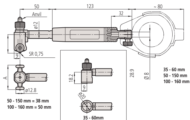
35 - 60mm
